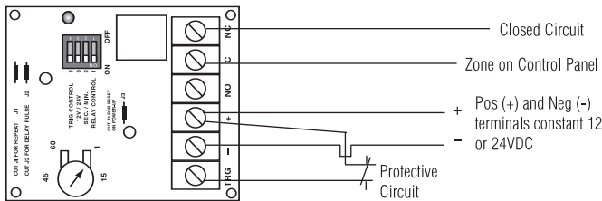
Fig. 3 - Swinger Eliminator:
